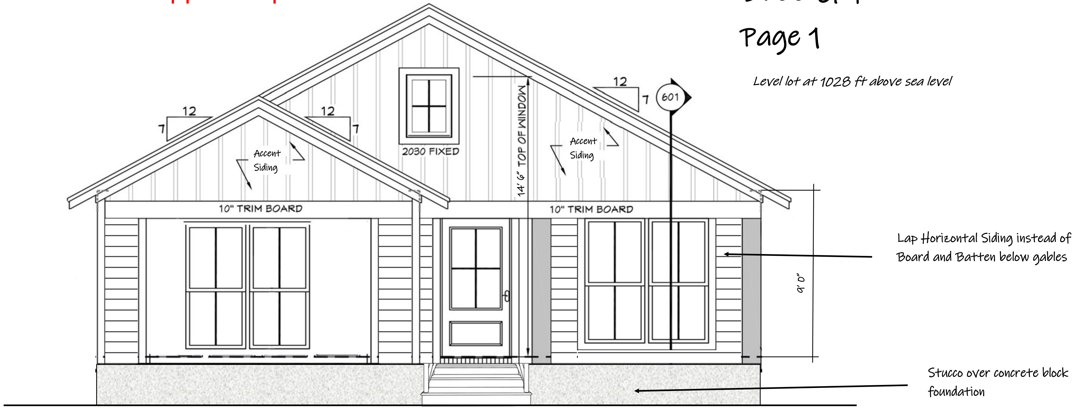
Front Elevation
