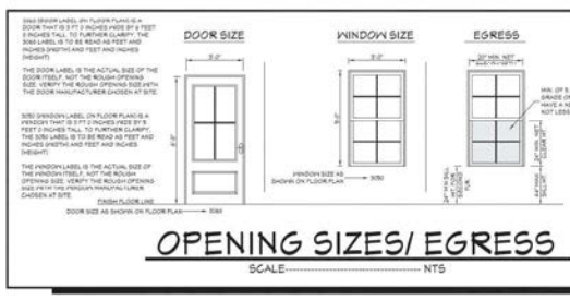
406 OPENING SIZES/ EGRESS SCALE: NTS
