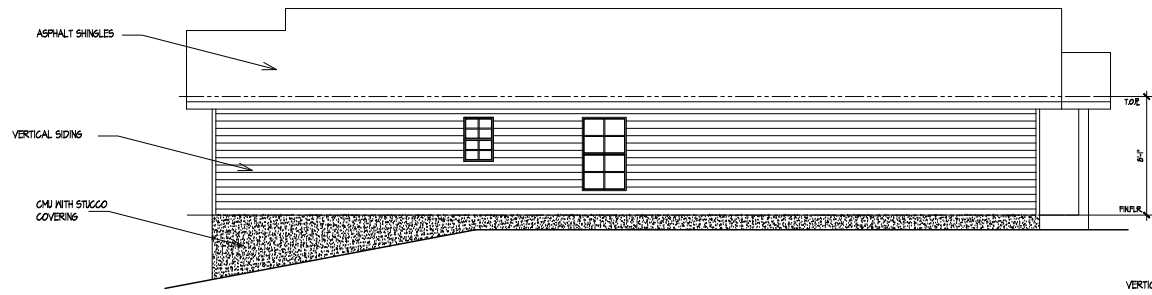
LEFT ELEVATION
