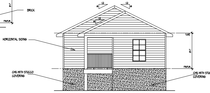
REAR ELEVATION
