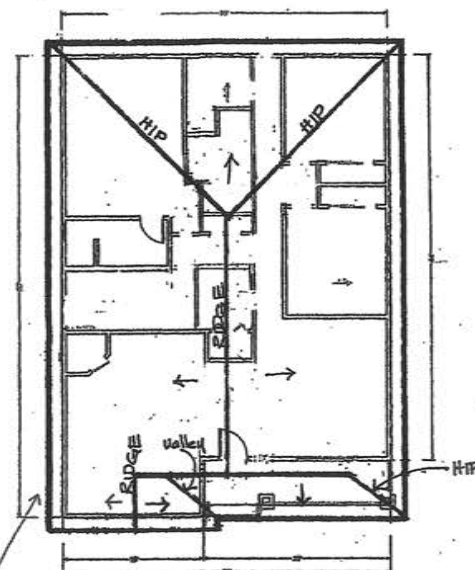
ROOF DESIGN HOUSE "C"
