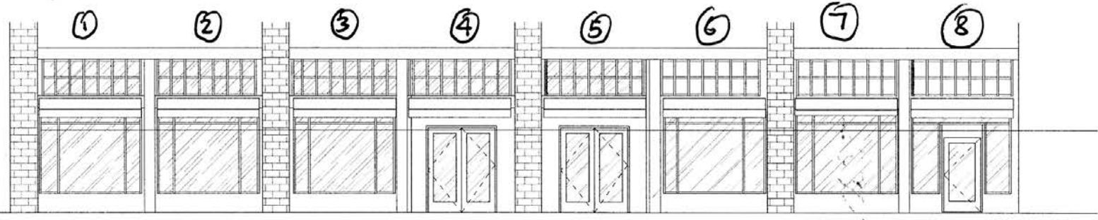
3 Gay St. ELEVATION 1/8" = 1'-0"
