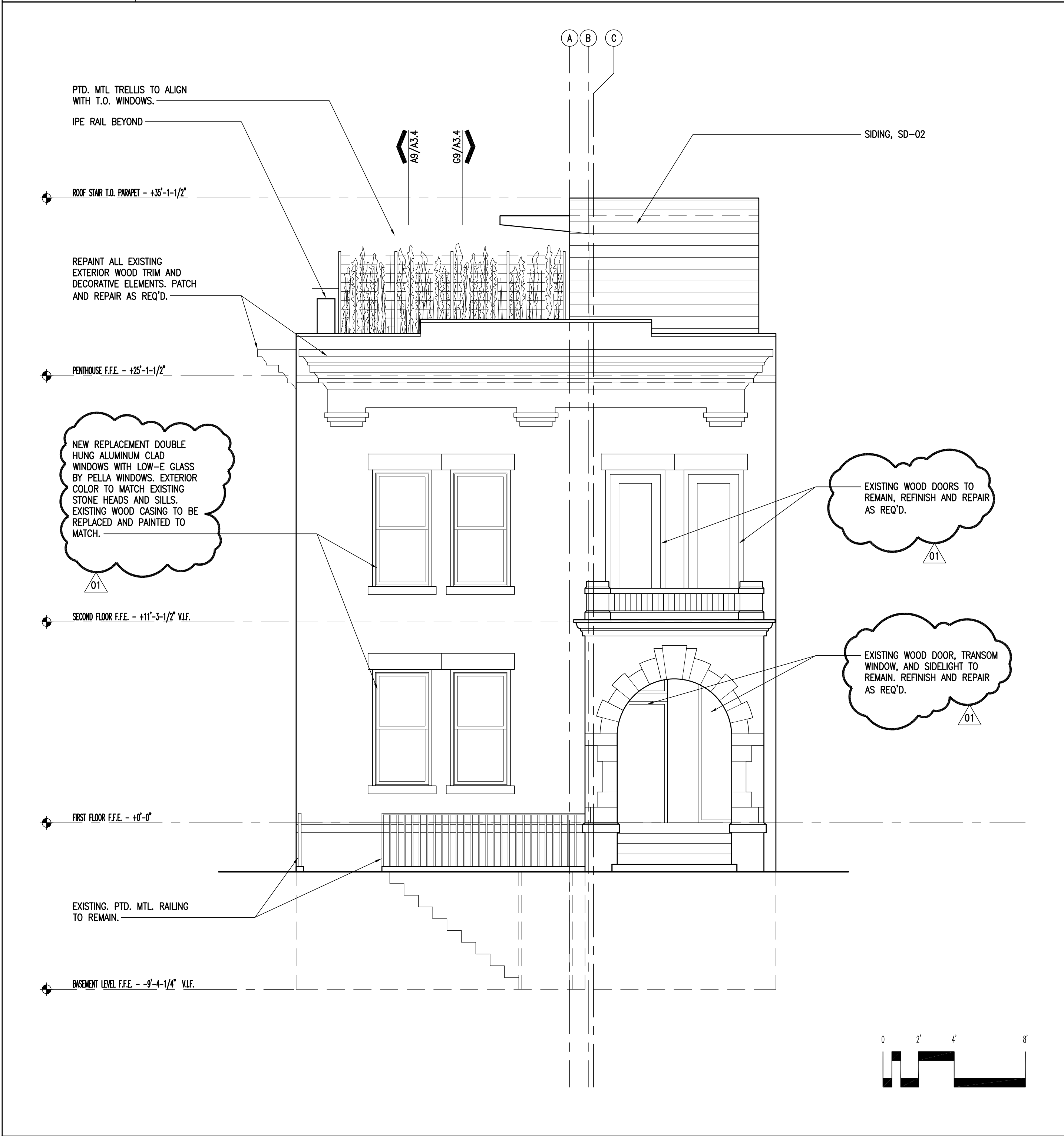
A1 NORTH ELEVATION 1339_XELEV 1/4" = 1'-0"
