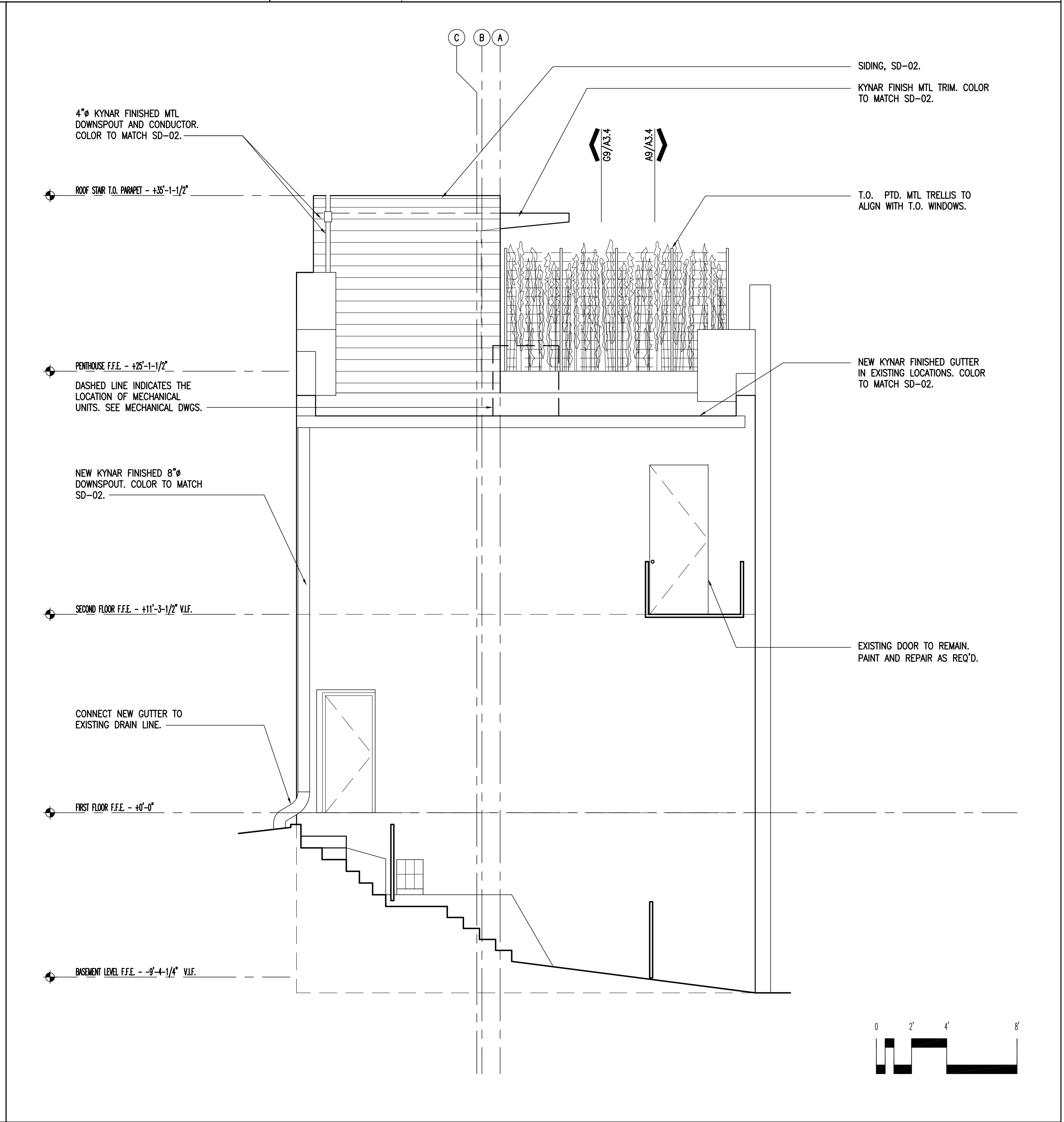
A9 SOUTH ELEVATION 1339_XELEV 1/4" = 1'-0"
