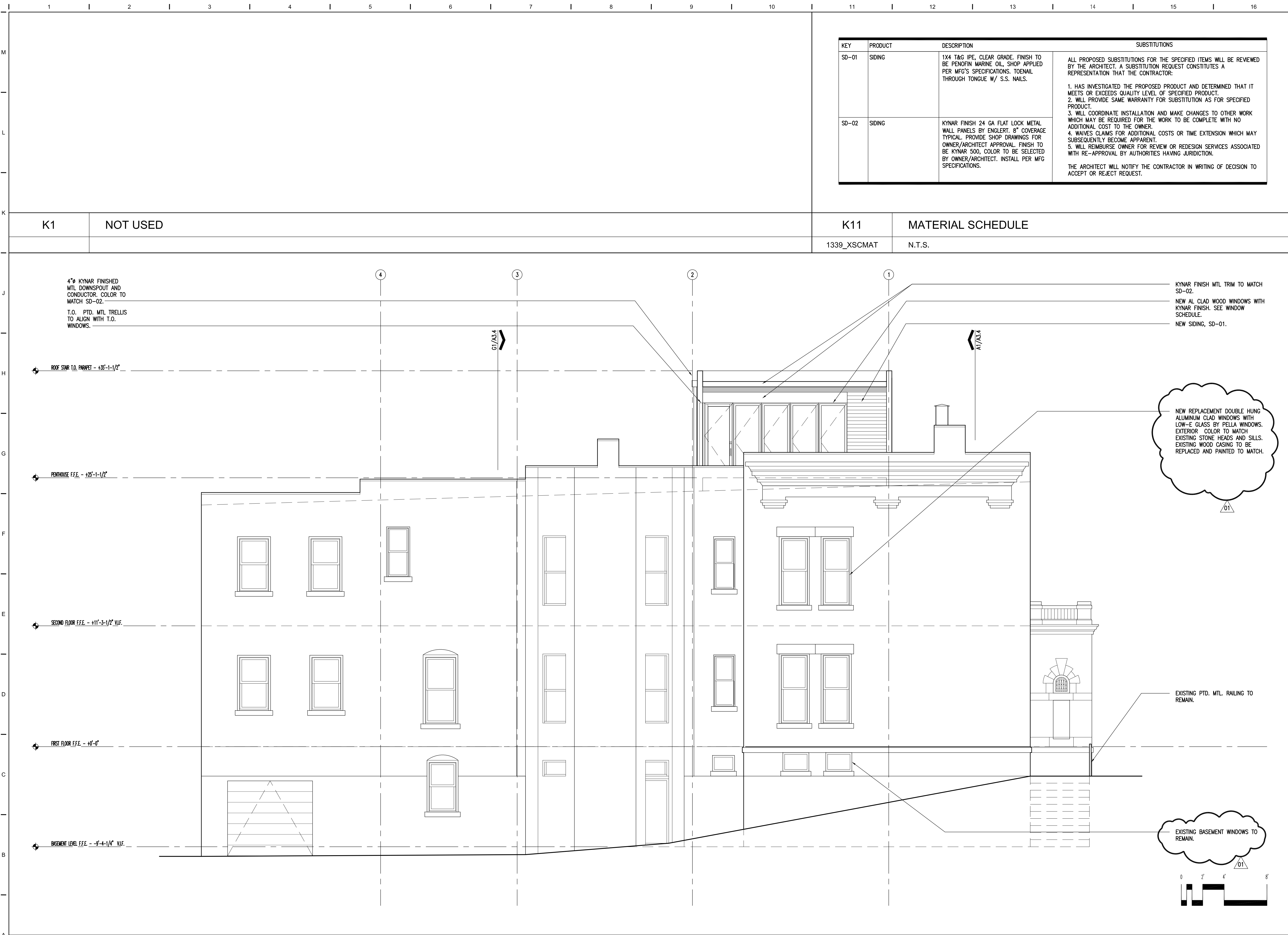
A1 EAST ELEVATION 1339_XELEV 1/4" = 1'-0"
