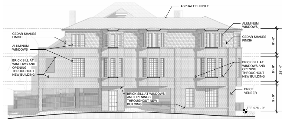
NORTH ELEVATION
